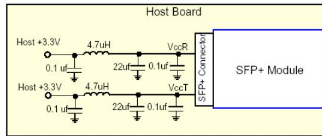
Figure 1: Recommended Host Board Power Supply Circuit
