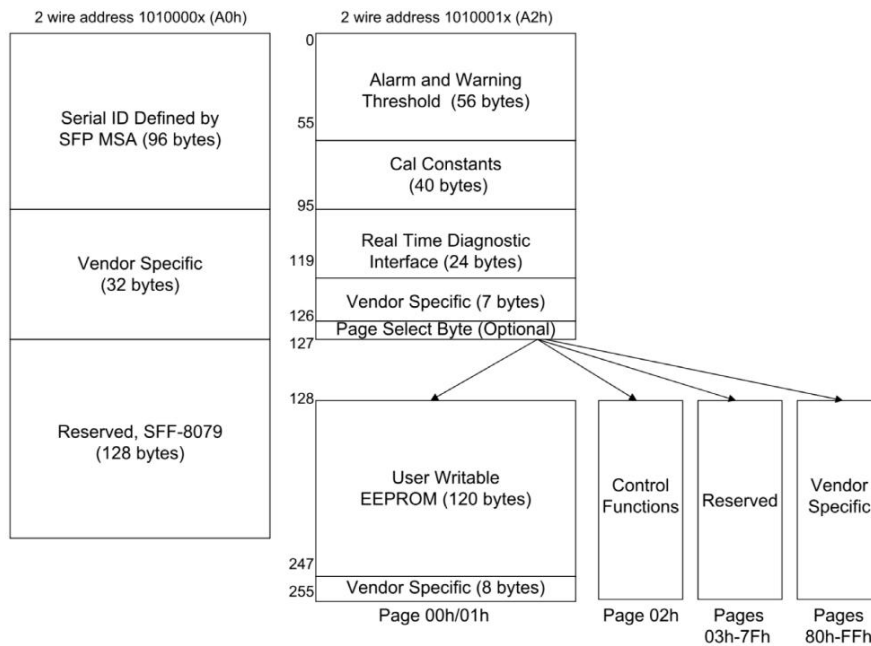
Figure4:Memory map
